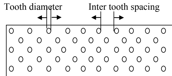
Figure 4.1: Grating Surface Dimensions
