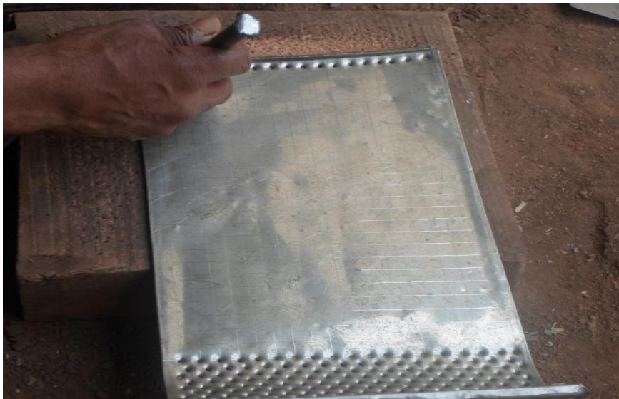
Figure 3.4: Punching process
